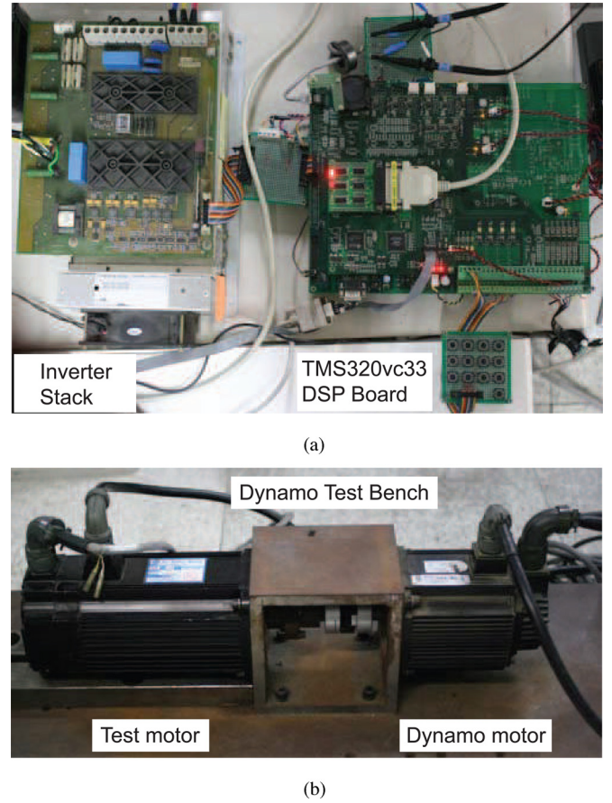
Fig. 5. Photos of the experiment setup. (a) Inverter for the test motor. (b) Dynamo test bench.
