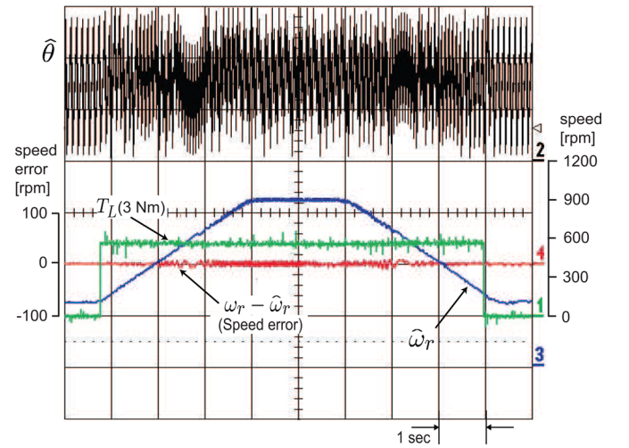
Fig. 10. Speed control response with a step full-load torque.
